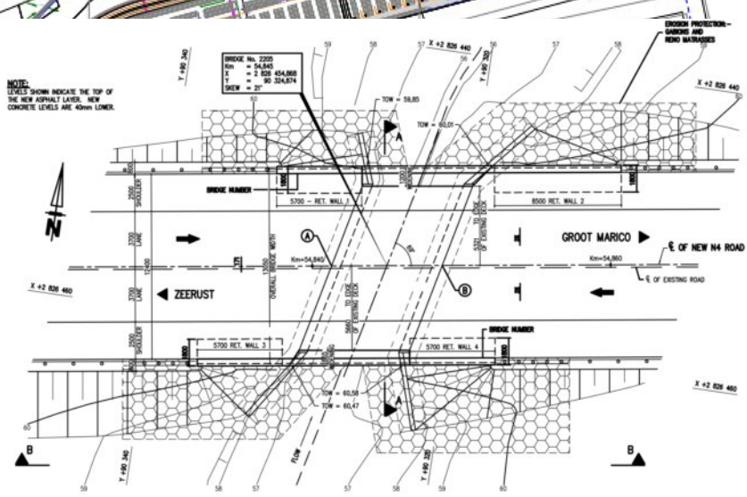
PLAN OF WIDENED BRIDGE SCALE 1:100
